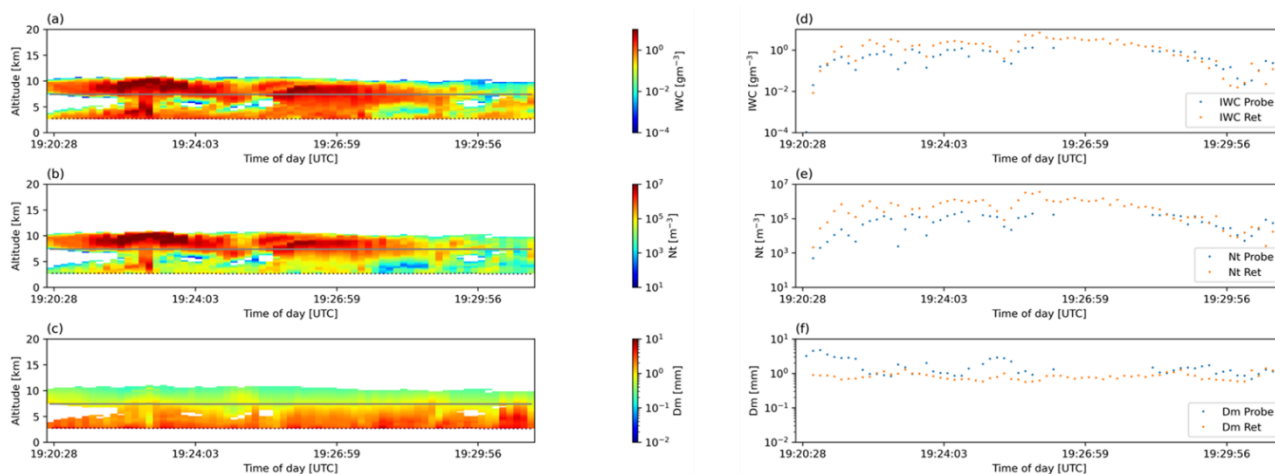
Figure 7: Same comparison as shown in Fig. 6, but for the deep convective rainfall case over the ocean on 25 January 2020
