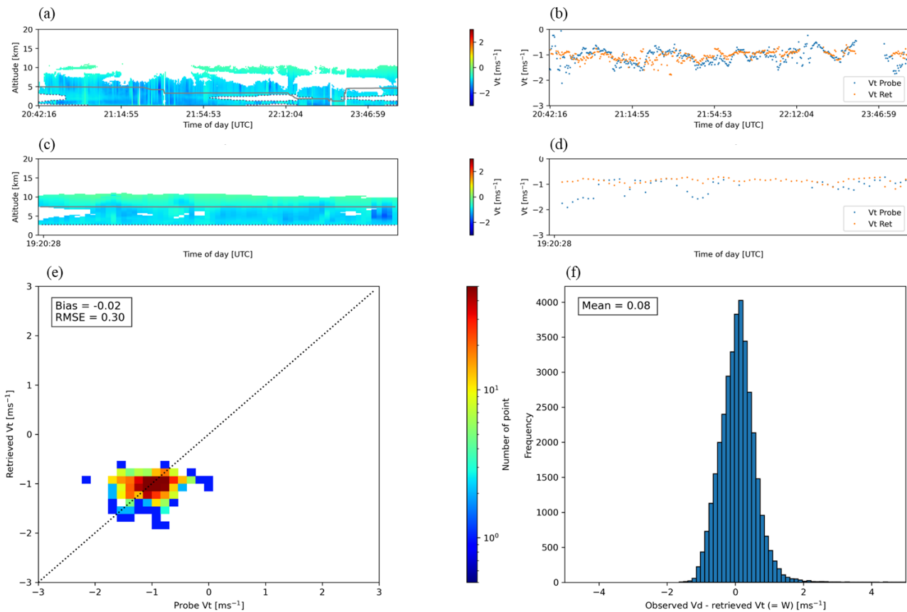
470 Figure 11 Evaluation of the retrieval accuracy for Z_w -weighted terminal fall velocity ( V_t ). (a) Vertical profiles of retrieved V_t and (b) comparison results between retrievals and probe measurements in the case shown in Fig. 6. (c) and (d) are same comparison as shown in (a) and (b), but for the case shown in Fig. 7. (e) Statistical comparison between retrieved and probe-measured V_t values across all cases. (f) Histogram of the difference between the CRS W-band Doppler velocity ( V_d ) and the retrieved V_t , corresponding to the vertical air motion W .
