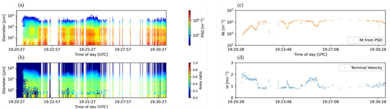
Figure 3: Example of in situ probe measurements from the P-3 aircraft. (a) Particle size distribution (PSD). (b) Area ratio ( A_r ) distribution. (c) Total number concentration ( N_t ) and (d) Z_w -weighted terminal fall velocity ( V_t ) calculated from the PSD in (a) and A_r in (b).
