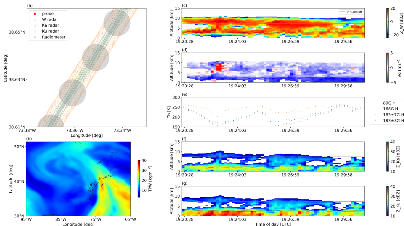
140 Figure 2: An example of observations by multiple sensors aboard the ER-2 aircraft on 25 January 2025. (a) Comparison of footprint sizes and sampling intervals among the ER-2-borne CoSMIR (radiometer), CRS (W-band radar), HIWRAP (Ku- and Ka-band radar), and the in-situ probes onboard the P-3 aircraft. (b) Flight track (black line) and the surrounding distribution of column-integrated water vapor (color map). (c) CoSMIR (nadir) brightness temperatures at 89, 165.5, and 183 \pm 3/7 GHz. (d) CRS W-band radar reflectivity. (e) CRS Doppler velocity. (f) HIWRAP Ku-band radar reflectivity. (g) HIWRAP Ka-band radar reflectivity. The gray solid line indicates the P-3 flight altitude, and the black dashed line indicates the 0^\circ\text{C} level.
