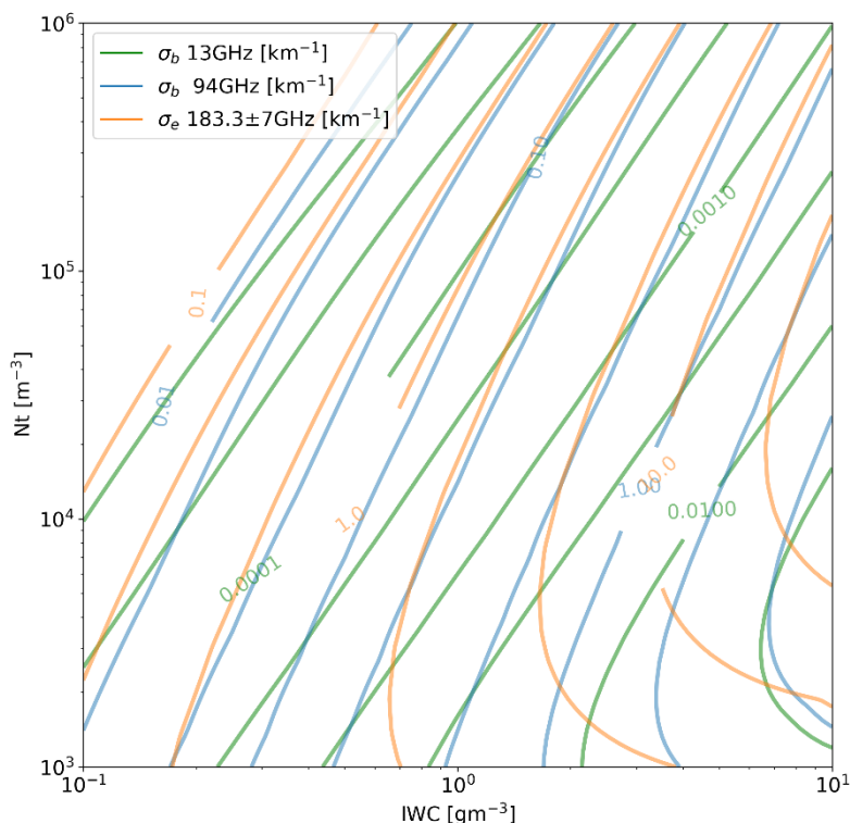
355 Figure 5: Sensitivity of the 13 GHz backscattering coefficient \sigma_{b13} (green), the 94 GHz backscattering coefficient \sigma_{b94} (blue), and the 183 \pm 7 GHz extinction coefficient \sigma_{e183 \pm 7} (orange).
